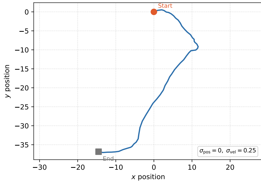
(b) Velocity noise only
